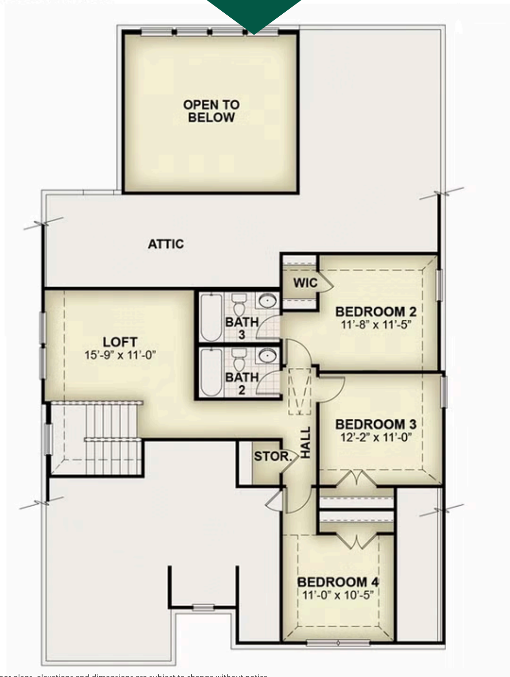
Second Floor
